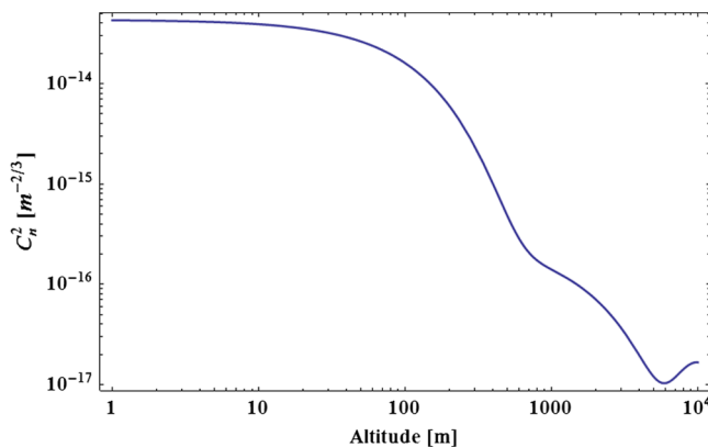
Fig. 8 Change in turbulence with altitude. Turbulence drops rapidly above 100 m.
