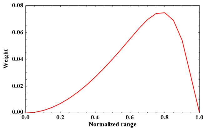
Fig. 7 Range-dependent path-weighting function of the influence of turbulence using the Kolmogorov spectrum. The source radius is 0.115 m, and the receiver radius is 0.01 m.
