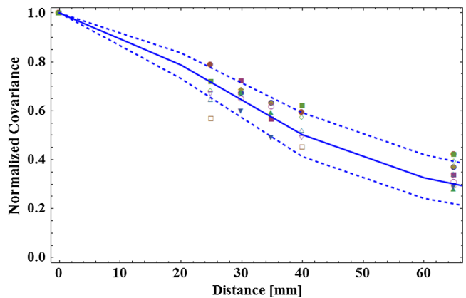
Fig. 6 Comparison of normalized covariance for a slant path from a building over an inhomogeneous area. The solid line shows the model prediction using a spectral power law parameter \alpha = 11/3 . The upper dashed line is for \alpha = 12/3 , and the lower dashed line is for \alpha = 10/3 . The turbulence levels varied between C_n^2 = 0.475 \times 10^{-14} and 2.43 \times 10^{-14} with a mean value of 1.40 \times 10^{-14} . The observations indicate that the similarity is high, at least under stable turbulence conditions. The range is L = 2,460 \text{ m} .
