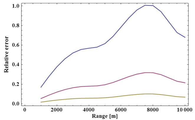
Fig. 9 Relative error (1 std) for a dual-aperture system with a diameter of 0.01 m separated by 0.025 m at turbulence levels of C_n^2 = 10 \times 10^{-14} \text{ m}^{-2/3} (upper curve), 1 \times 10^{-14} \text{ m}^{-2/3} (middle curve), and 0.1 \times 10^{-14} \text{ m}^{-2/3} (lower curve) as a function of range.
