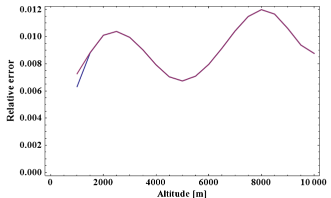
Fig. 10 Relative error (1 std) for a dual-aperture system with a diameter of 0.01 m separated by 0.025 m at a turbulence level of C_n^2 = 100 and 1 \times 10^{-14} \text{ m}^{-2/3} as a function of altitude. For altitudes above 1,500 m, the relative error is independent of ground level turbulence, and the two curves are superimposed on each other. For low altitudes, a higher level of turbulence will result in a higher relative error.
